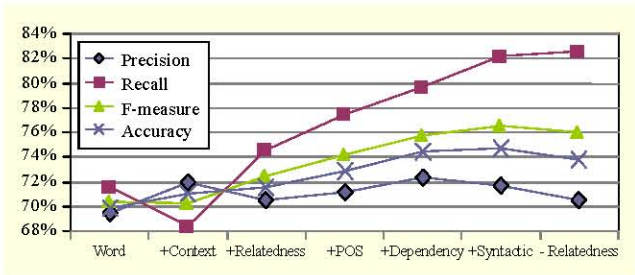
Fig. 1. Contribution of each feature set for isa relation type.
