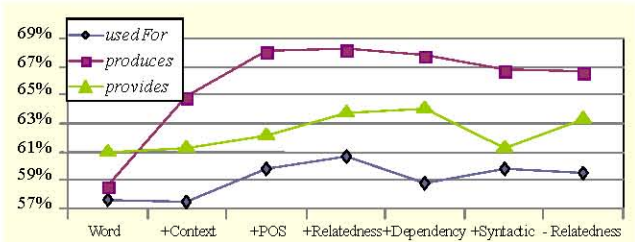
Fig. 2. Feature evaluation on other three relation types with F-measure.
