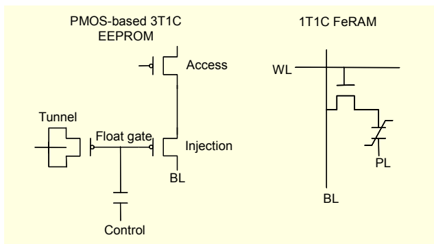
Fig. 1. PMOS-based EEPROM cell and FeRAM cell.
