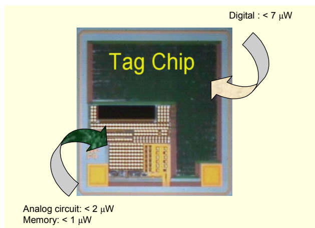
Fig. 8. Measured read and write power consumption of FeRAM-embedded RFID chip.
